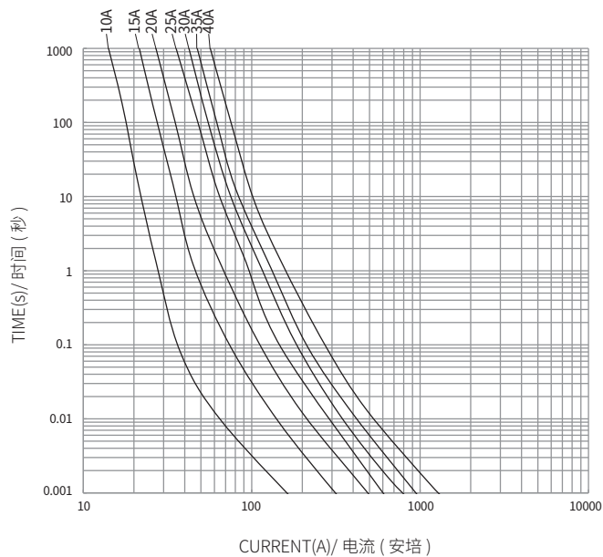
HC107EV-T 平均 I-T 曲线图 (仅供参考) AVERAGE I-T CHARACTERISTICS CURVE (FOR REFERENCE ONLY)
